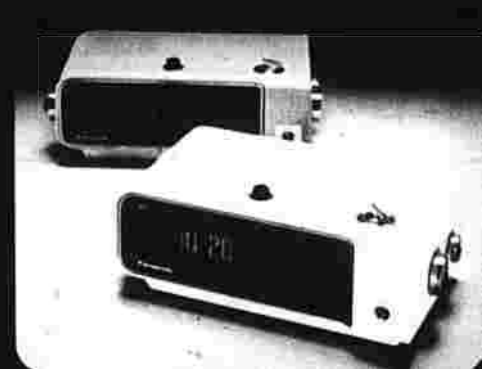
RC-6003 FM/AM Digital Clock Radio. 24-hour digital clock. 60-minute sleep timer. Automatic shut-off. Music or buzzer alarm. Lighted digital clock. 2 \frac{1}{2} " speaker. FM external antenna terminal. Solid-state. In antique white or beige. RC6003/3995 ..... Retail $49.95
